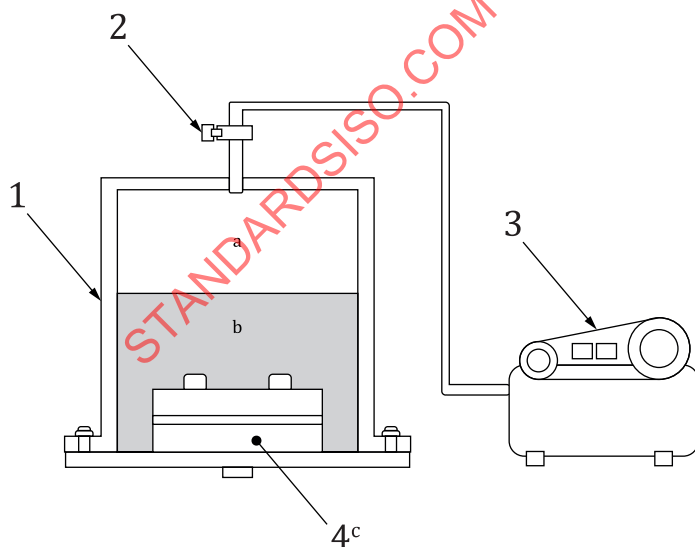
a) Permeability test chamber (output)
