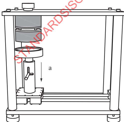
c) Step 3 Lower the supporting plate
