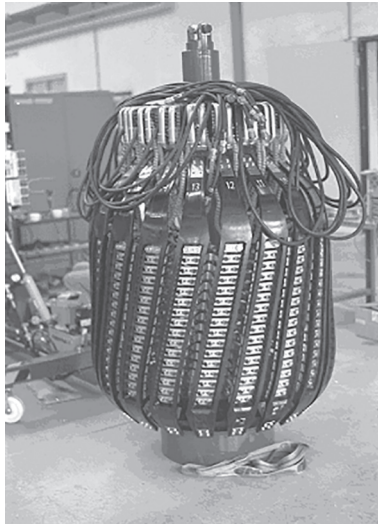
Figure 3 — Probe assembly of an intelligent pig for use on a 40-inch-diameter pipeline
