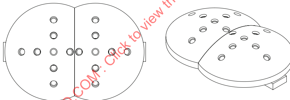
Figure 5 — Indenter assembly for 380 mm indenter
