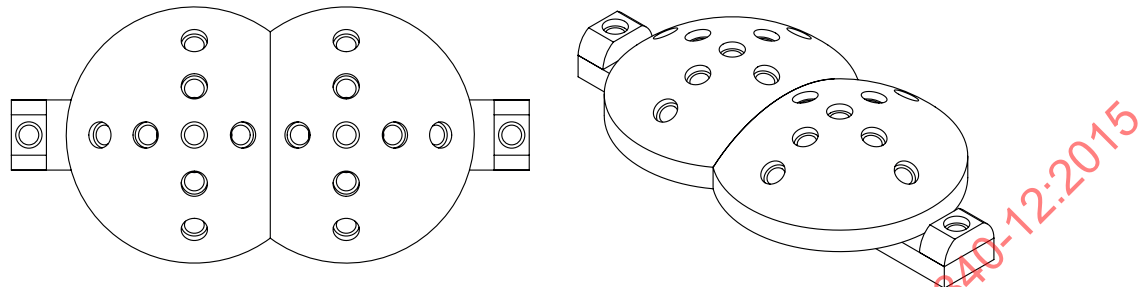
Figure 4 — Indenter assembly for 220 mm and 255 mm indenters
