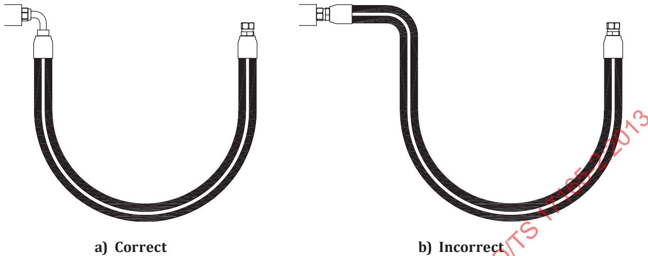
Figure 3 — Elbows and connectors
