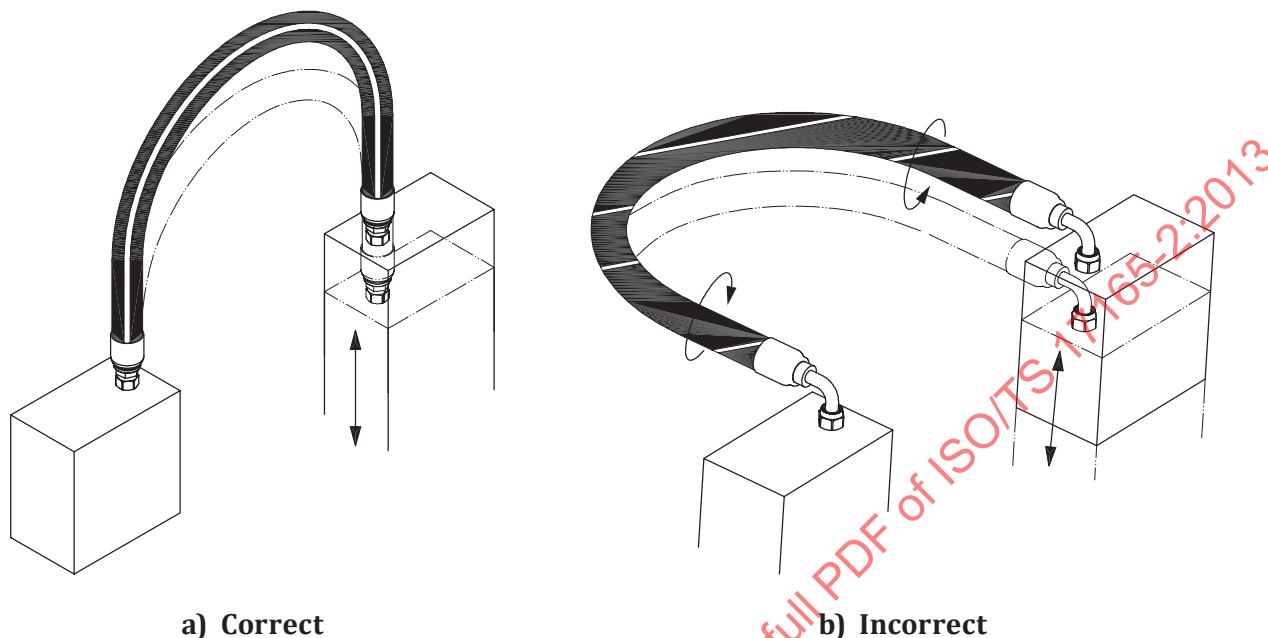
Figure 7 — Illustration of bending in only one plane to avoid twisting
