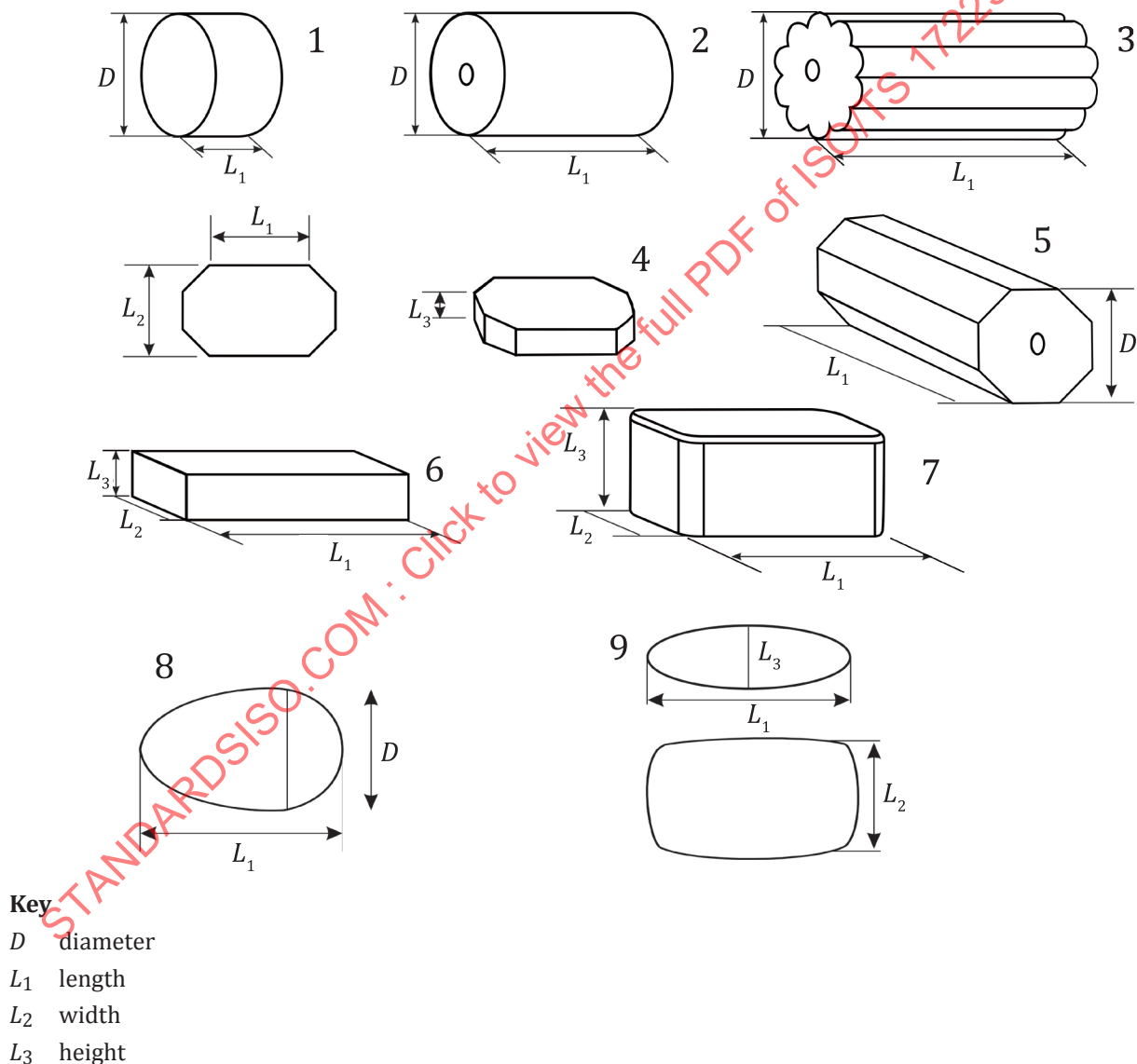
Figure 2 — Examples of briquette shapes with associated dimensions
