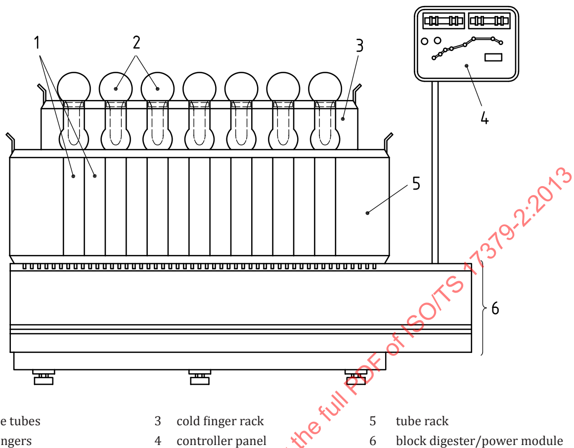
Figure B.3 — An example of a suitable block digester with the cold finger arrangement
