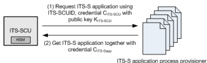
Figure 9 — ITS-S application process provisioning — Functional illustration
