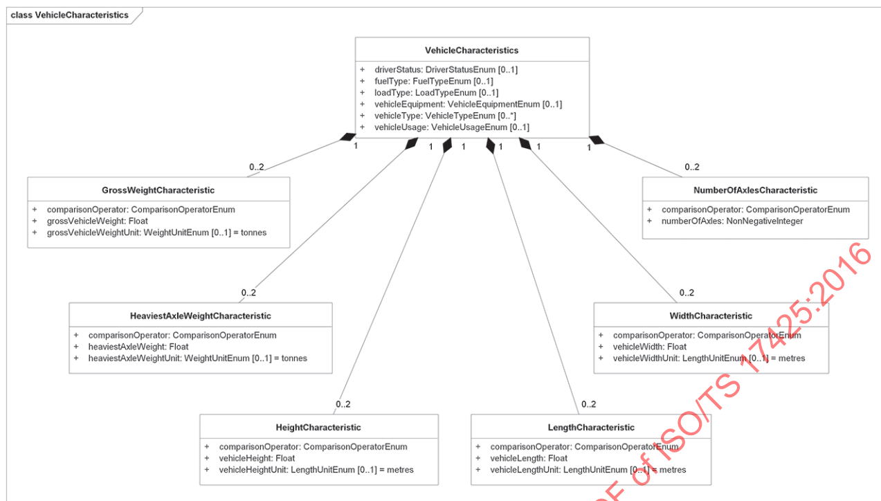
Figure A.9 — “VehicleCharacteristics” package
