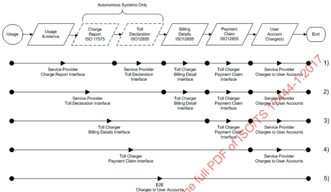
Figure 5 — Charging Metrics mapping to toll scheme Implementations
