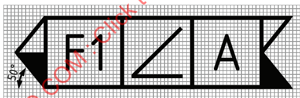
Figure A.2 — Force indicator including basic indication of specific direction of the force relative to a datum
