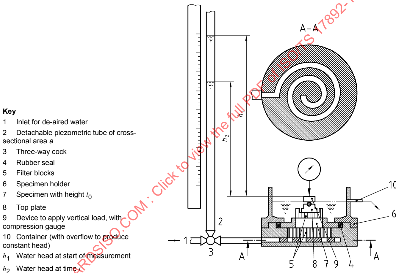
Figure 4 — Example for a test arrangement for compression permeameter test
