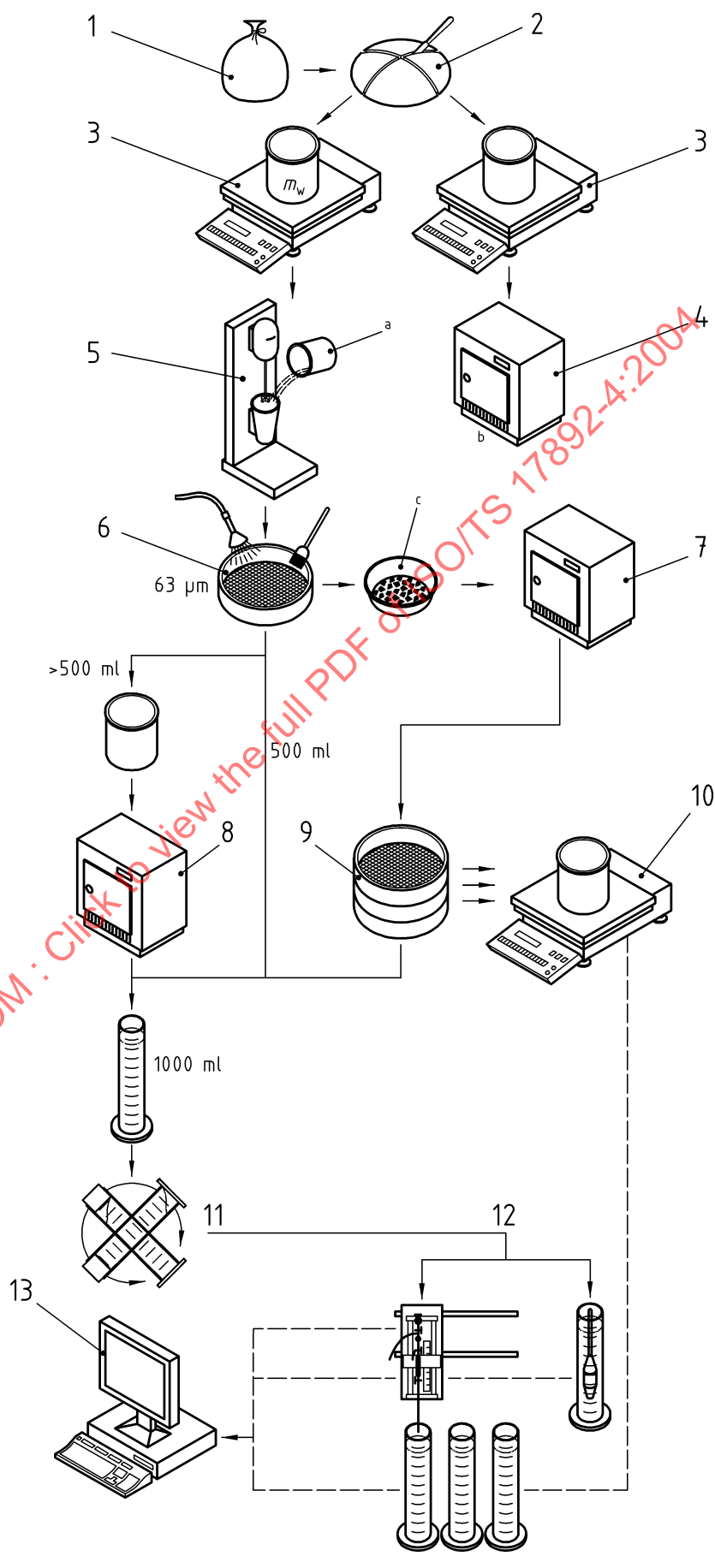
Figure 3 — General procedure for sedimentation
