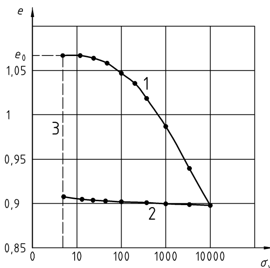
Figure 2 — Typical plot of void ratio against vertical effective stress
