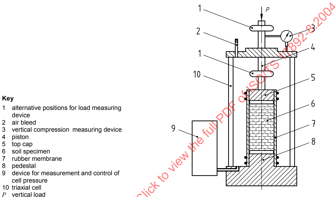
Figure 1 — Example of a triaxial test unit
