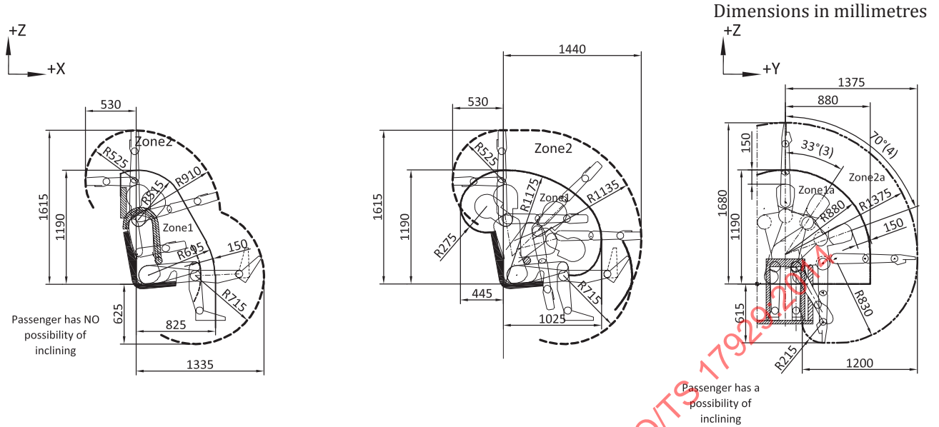
Figure A.4 — Zone of potential biomechanical risks in reach envelopes for passengers in a sitting position, along y-axis (sideward)
