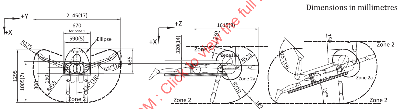
Figure A.3 — Zone of potential biomechanical risks in reach envelopes for passengers in a prone position, along Z-axis (back and forward)
