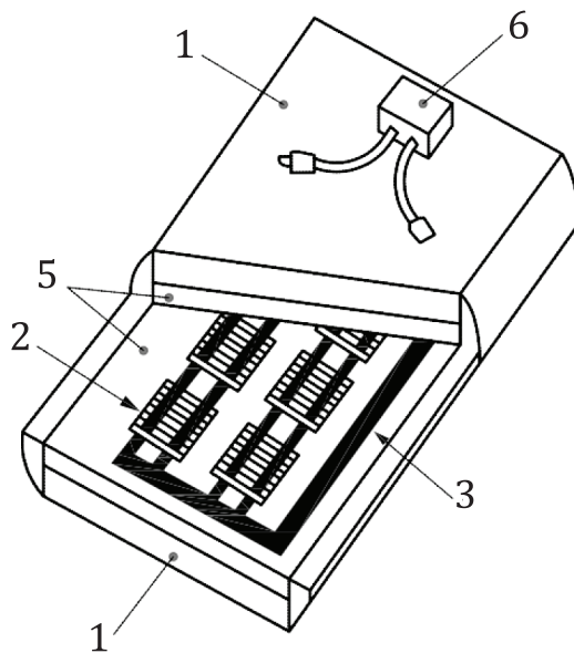
a) Crystalline silicon type laminated solar PV glass
