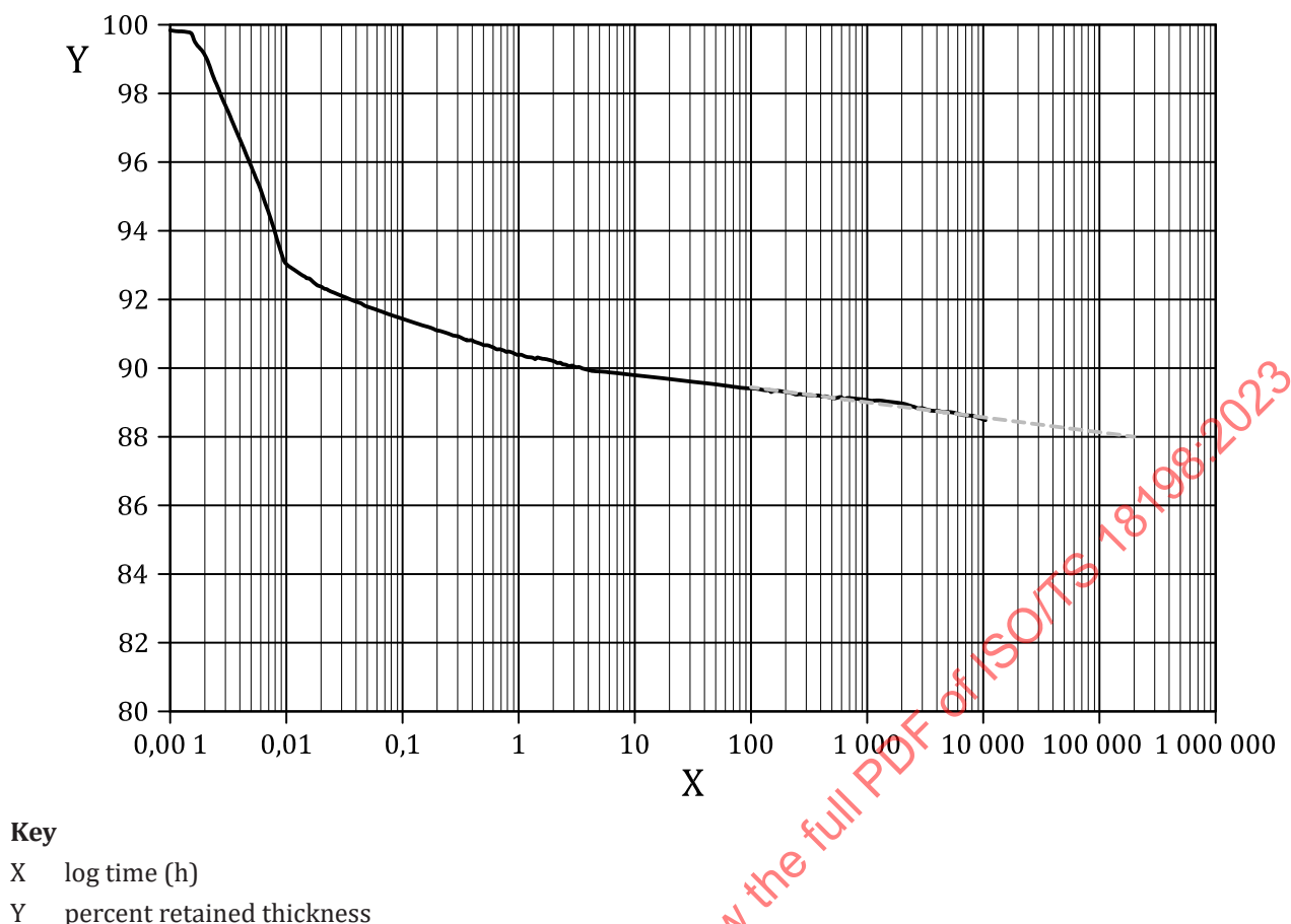
Figure 4 — Example of compressive creep curve for a drainage core
