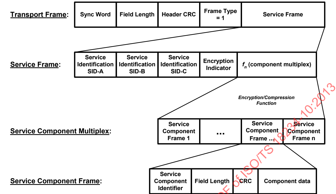
Figure A.3 — TPEG Frame Structure, Frame Type = 1 (i.e. conventional data)
