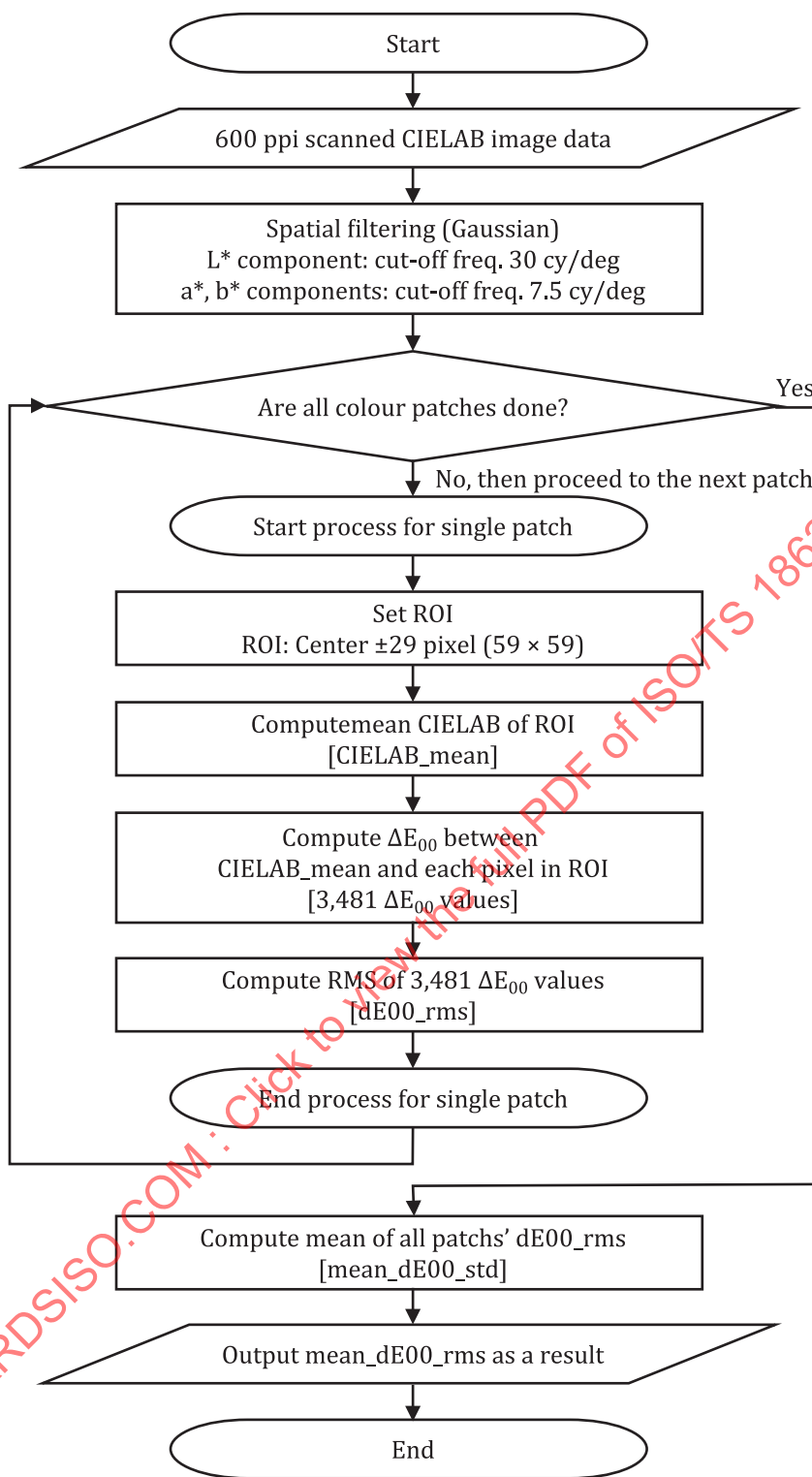
Figure 1 — Computation flowchart
