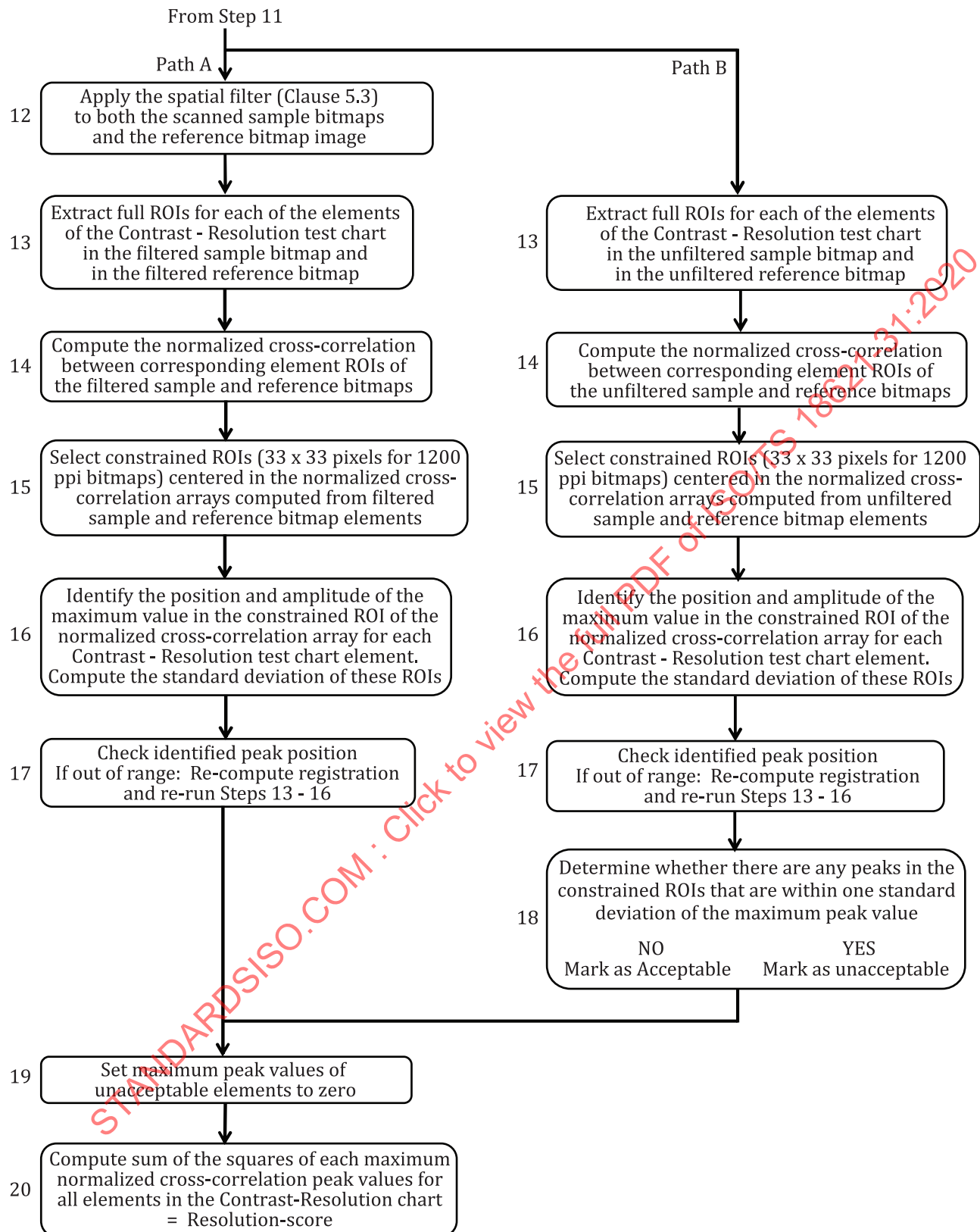
Figure 8 — Flow-chart of steps 12 through 20 of resolution-score analysis
