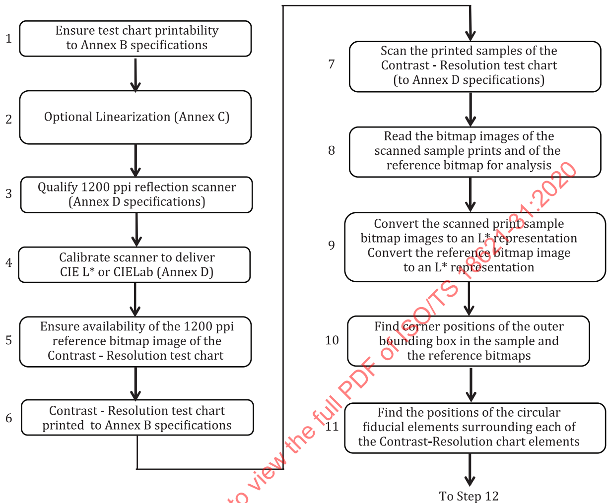
Figure 7 — Flow-chart of Steps 1 through 11 in resolution-score analysis
