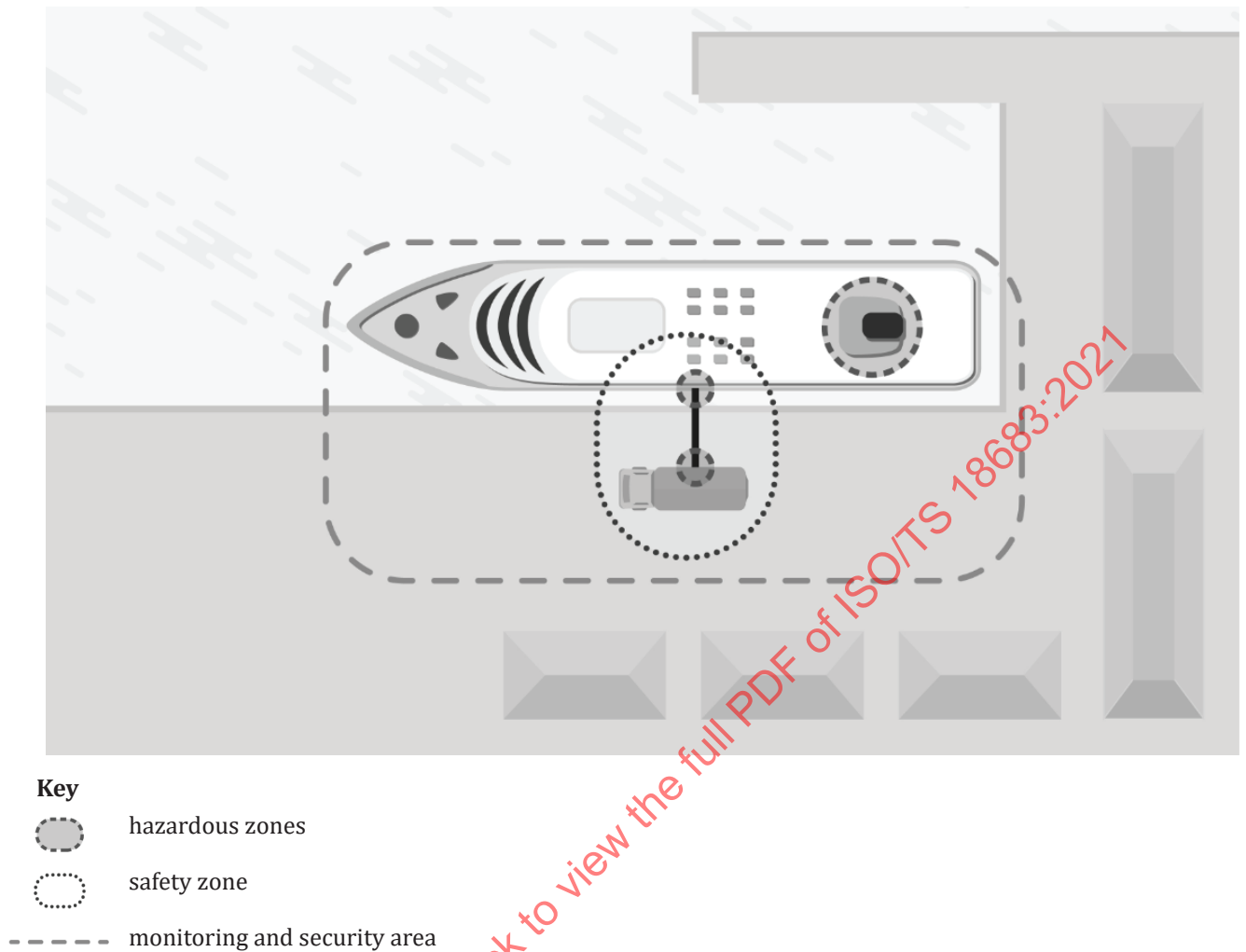
Figure 2 — Safety zone and controlled areas
