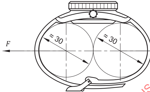
Figure 1 — Representation of the test for resistance of attachments
