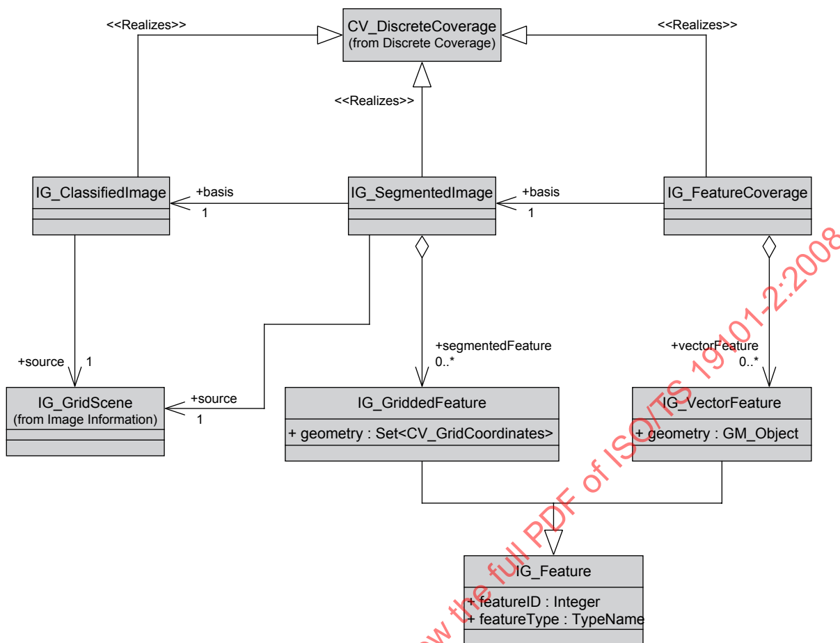
Figure 13 — Image classification and understanding class diagram
