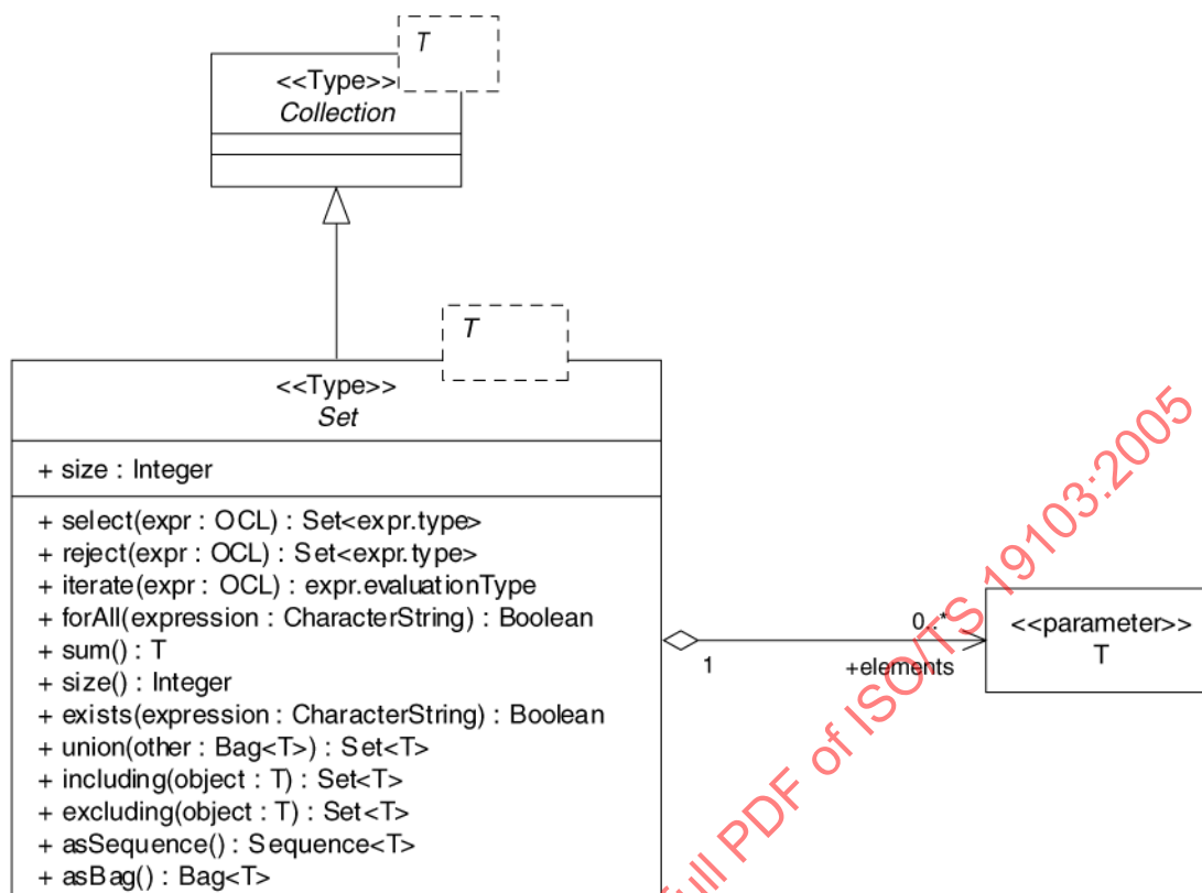
Figure 9 — Collection types — Set type
