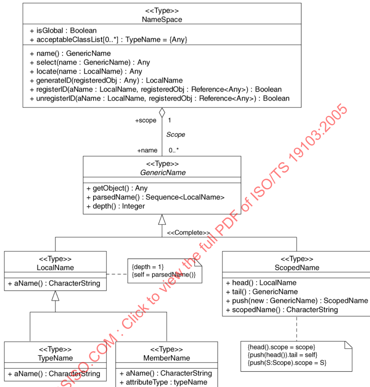
Figure 16 — Name types
