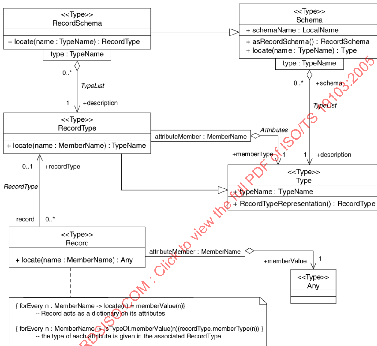
Figure 15 — Record types
