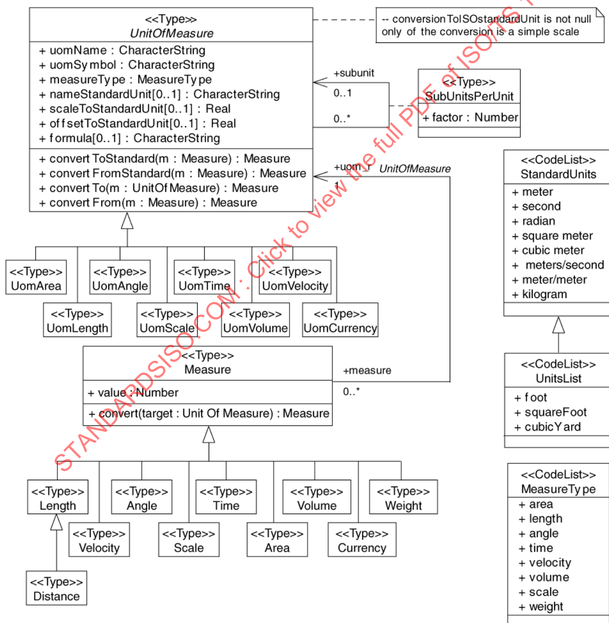
Figure 17 — Units of Measure types
