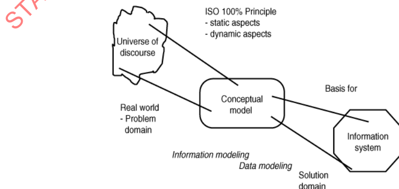
Figure B.3 — The ISO 100 % principle for conceptual modeling
