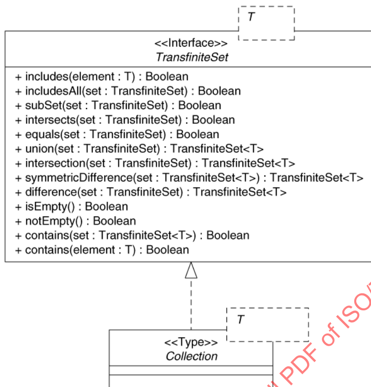
Figure 8 — Collection type
