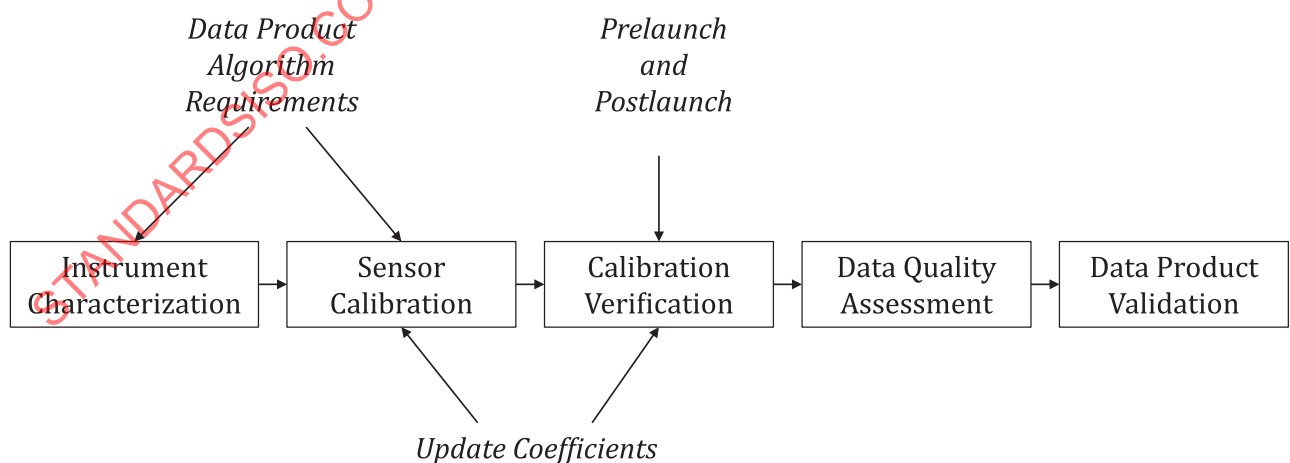
Figure 12 — Five key steps from prelaunch sensor calibration to on-orbit data product validation [3]
