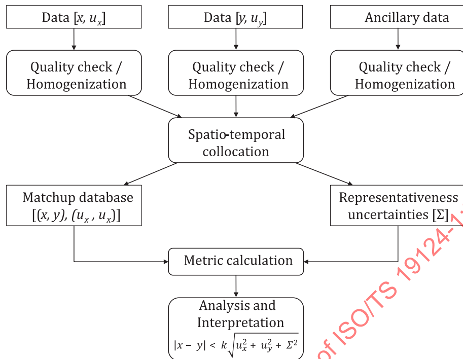
Figure 9 — Schematic overview of the general validation process [6]
