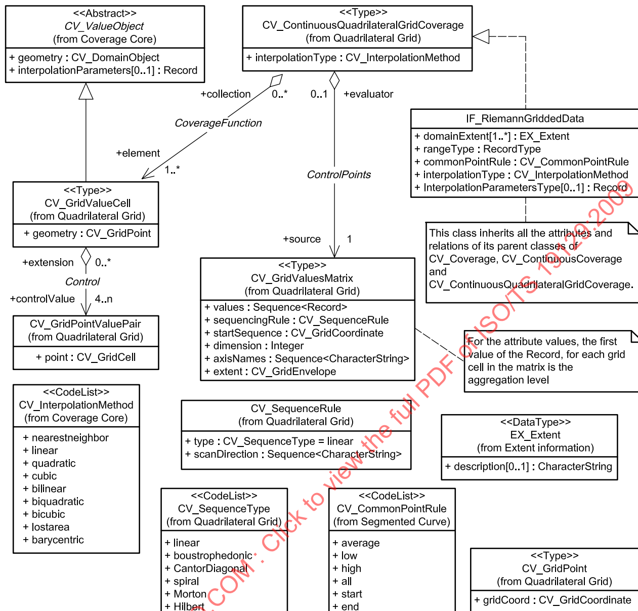
Figure 12— Template application schema for Riemann grid coverage
