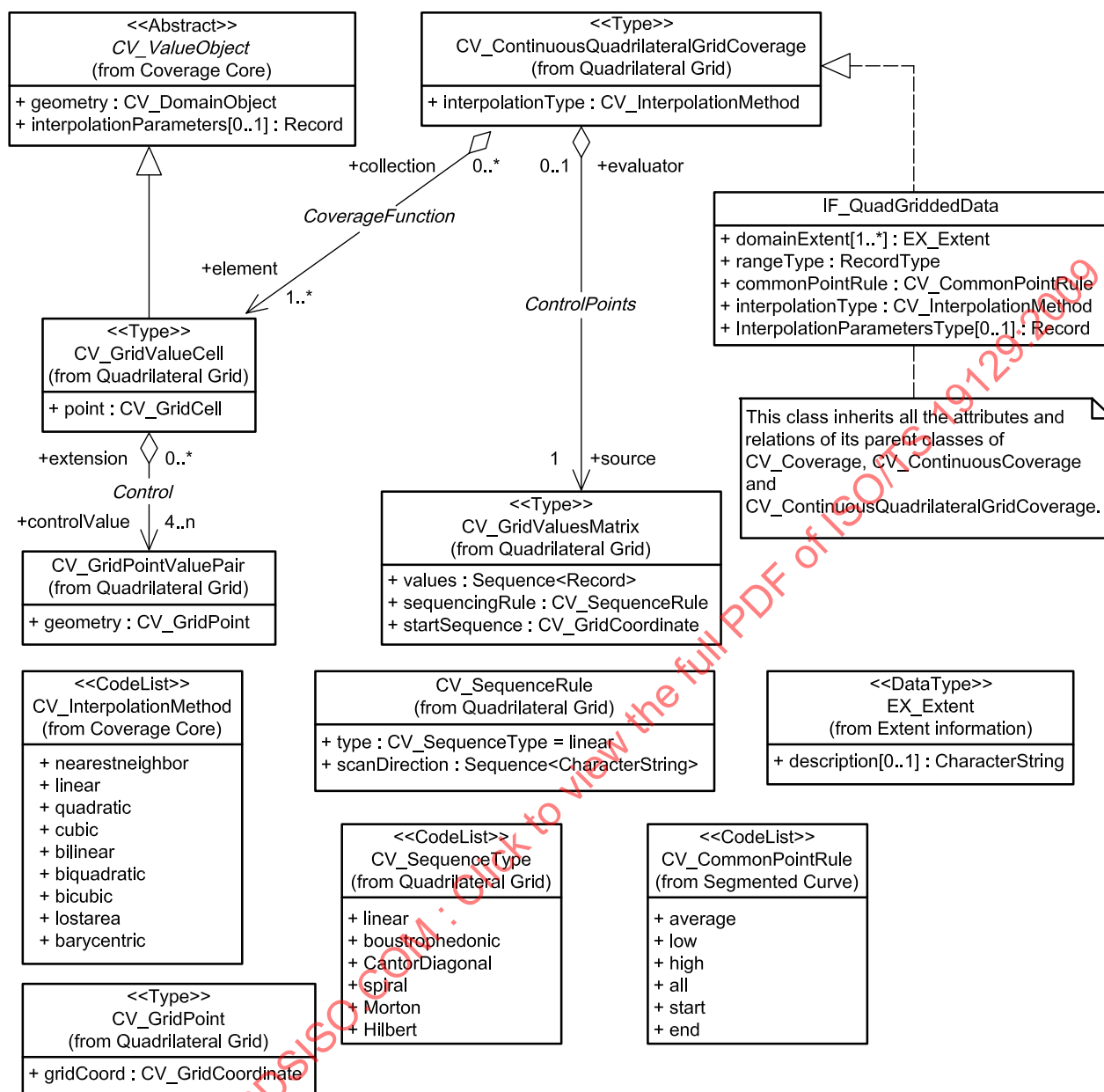
Figure 11 — Template application schema component for a quadrilateral grid
