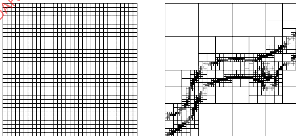
Figure 8 — Regular and variable cell size grids
