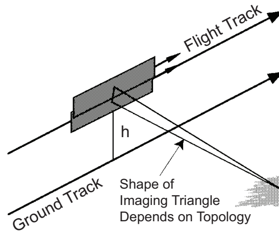
Figure 6 — Cross-track InSAR Configuration (from Rosen et al., 2000)
