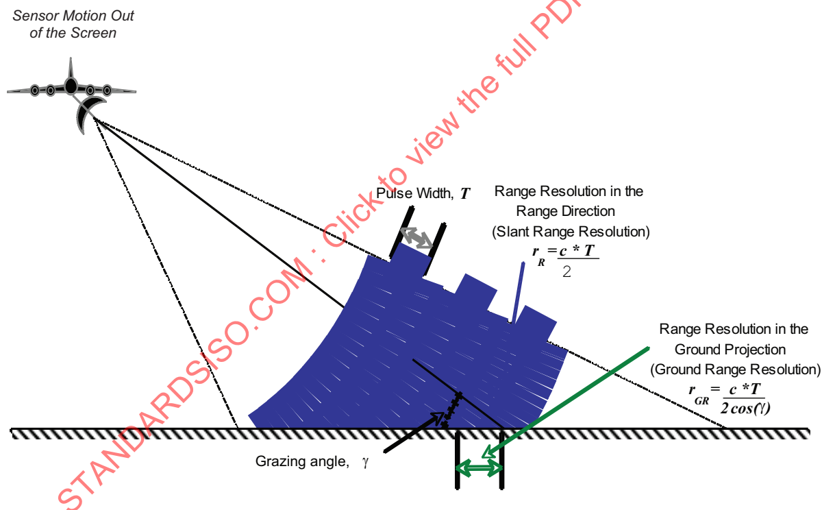
Figure C.9 — Slant Range Resolution vs. Ground Range Resolution
