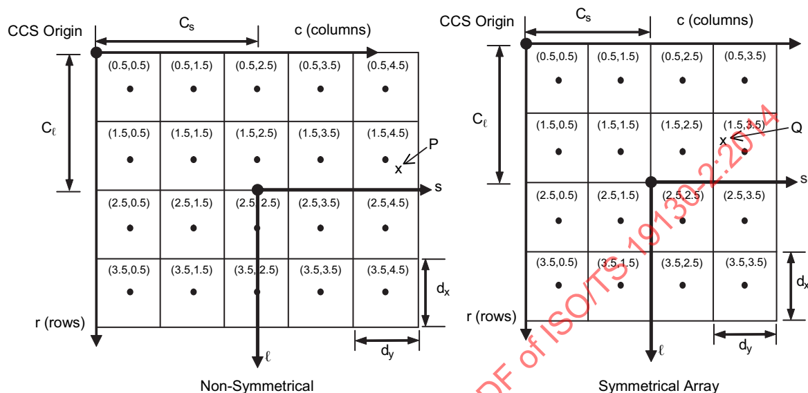
Figure C.6 — Pixel orientation within the frame sensor coordinate system
