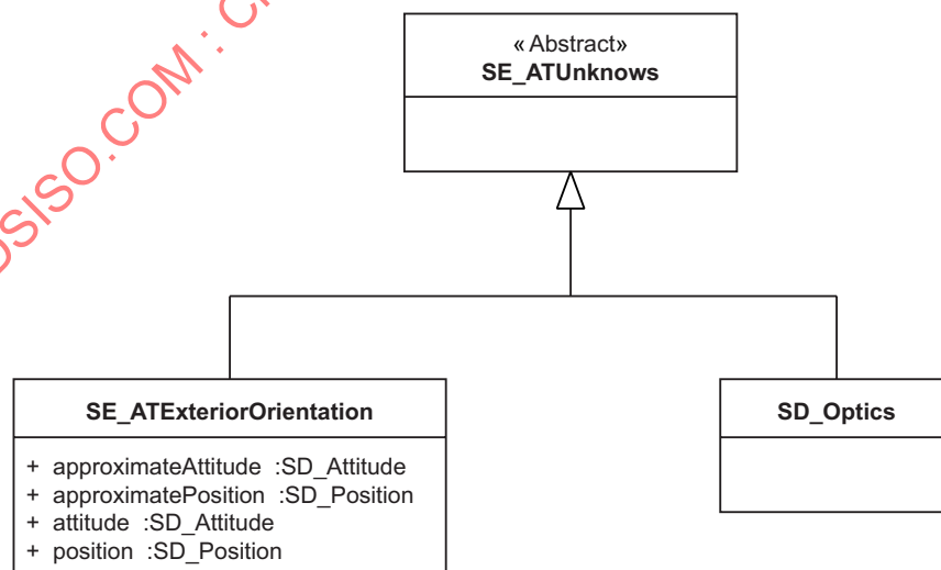
Figure 24 — Exterior orientation of aerial triangulation
