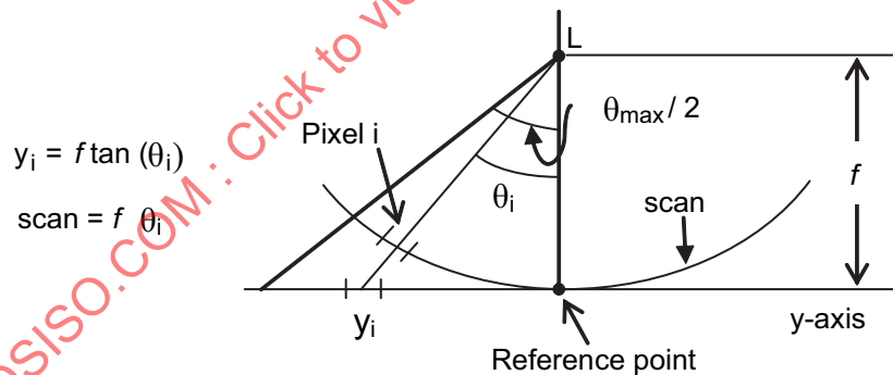
Figure C.11 — Whiskbroom sensor model
