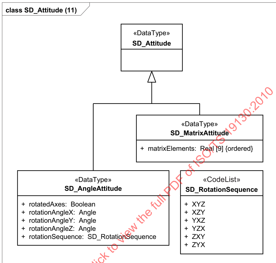
Figure 11 — SD_Attitude
