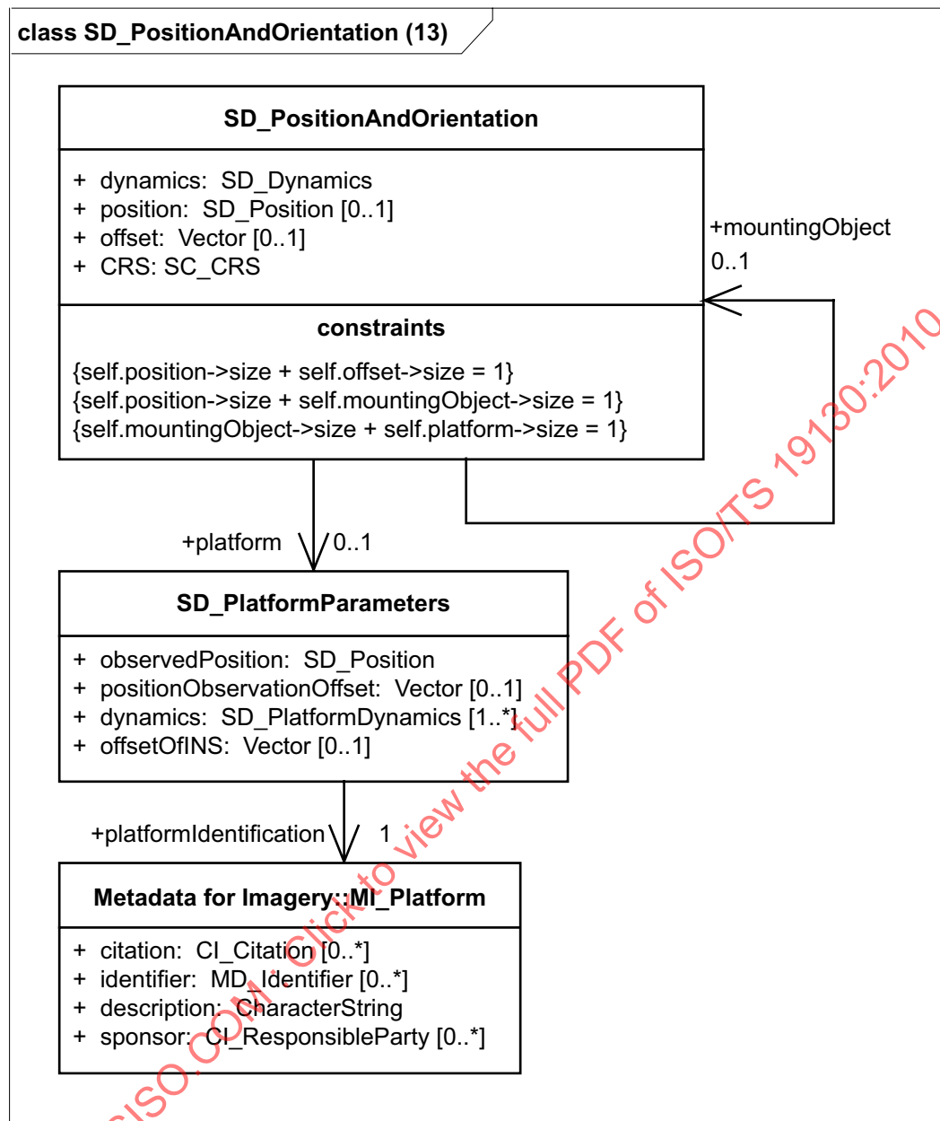
Figure 13 — SD_PositionAndOrientation
