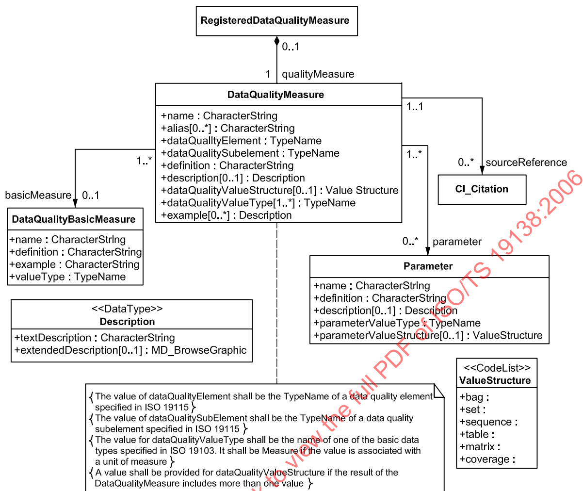
Figure B.1 — Data quality measure
