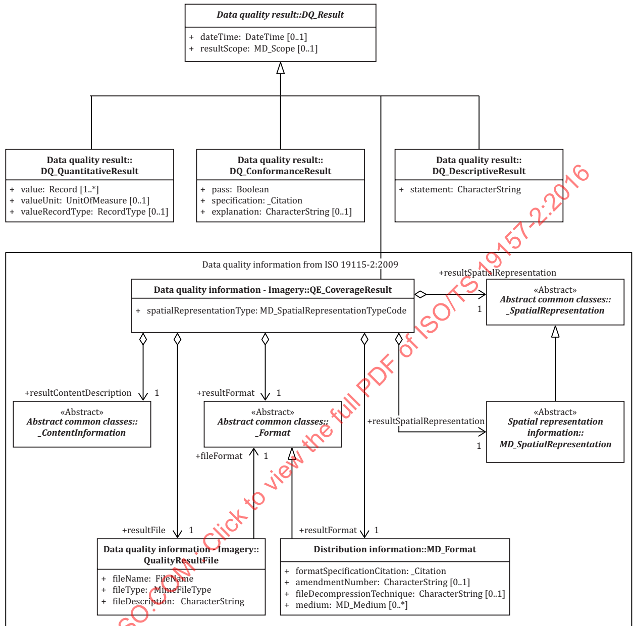
Figure C.1 — ISO 19115-2:2009-parts in DQ_Result (UML class diagram)
