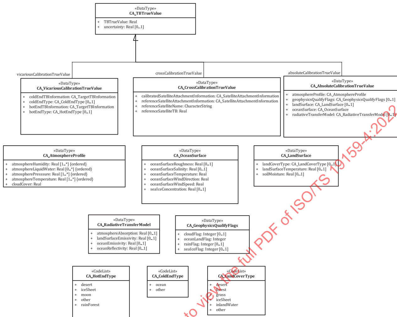
Figure 9 — CA_TBTrueValue class diagram
