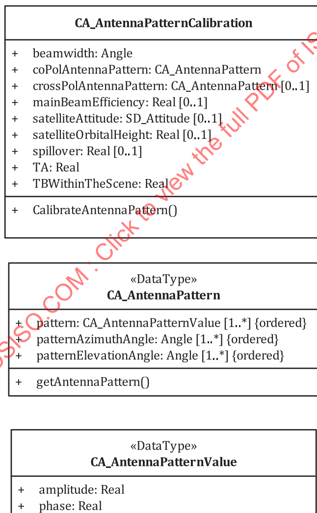
Figure 6 — CA_AntennaPatternCalibration class diagram
