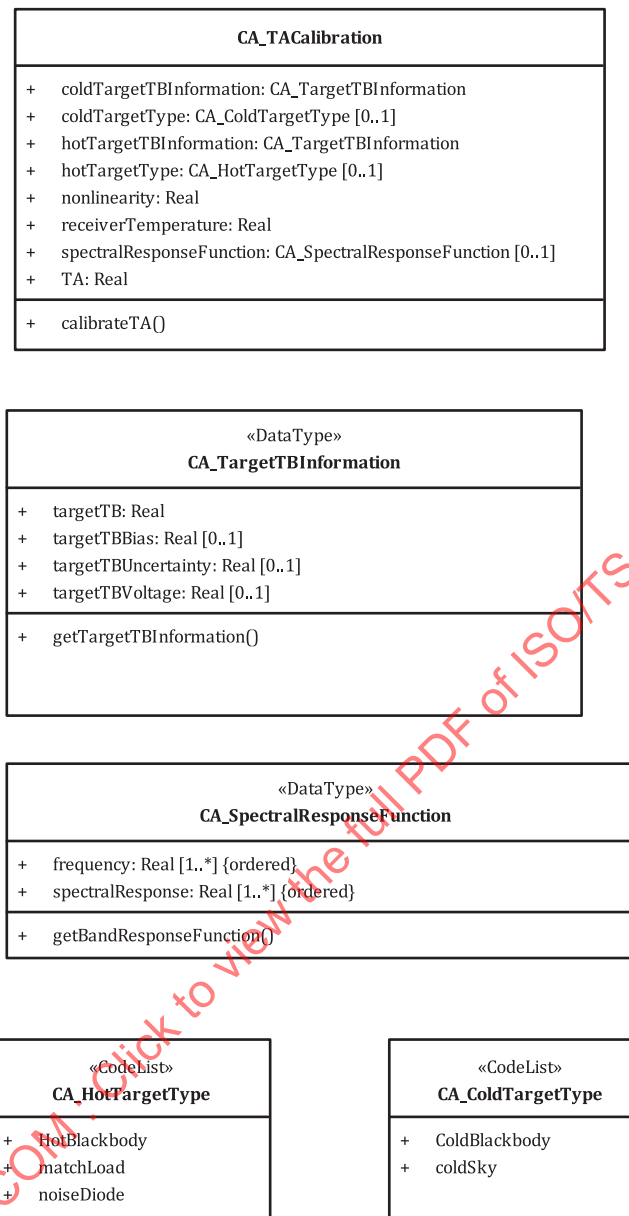
Figure 5 — CA_TACalibration class diagram
