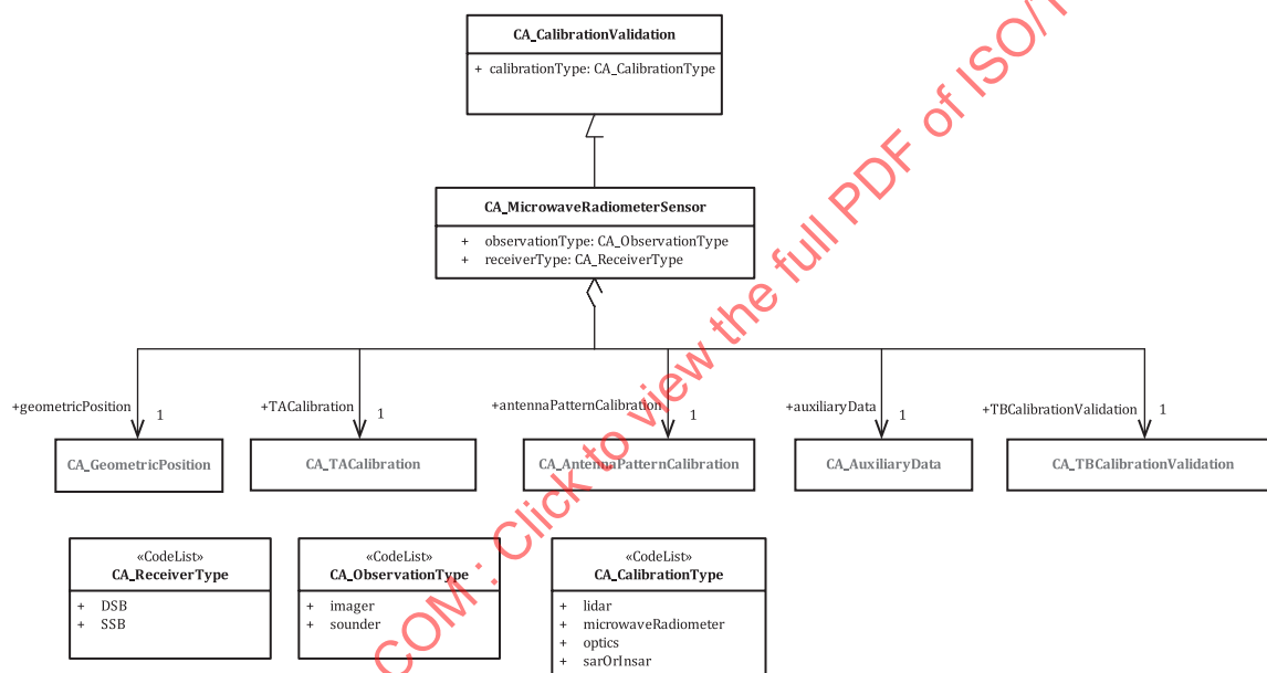
Figure 3 — Class diagram of ISO/TS 19159-4 (this document)
