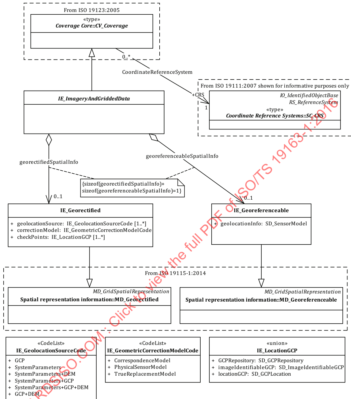
Figure 3 — IE_ImageryAndGriddedData
