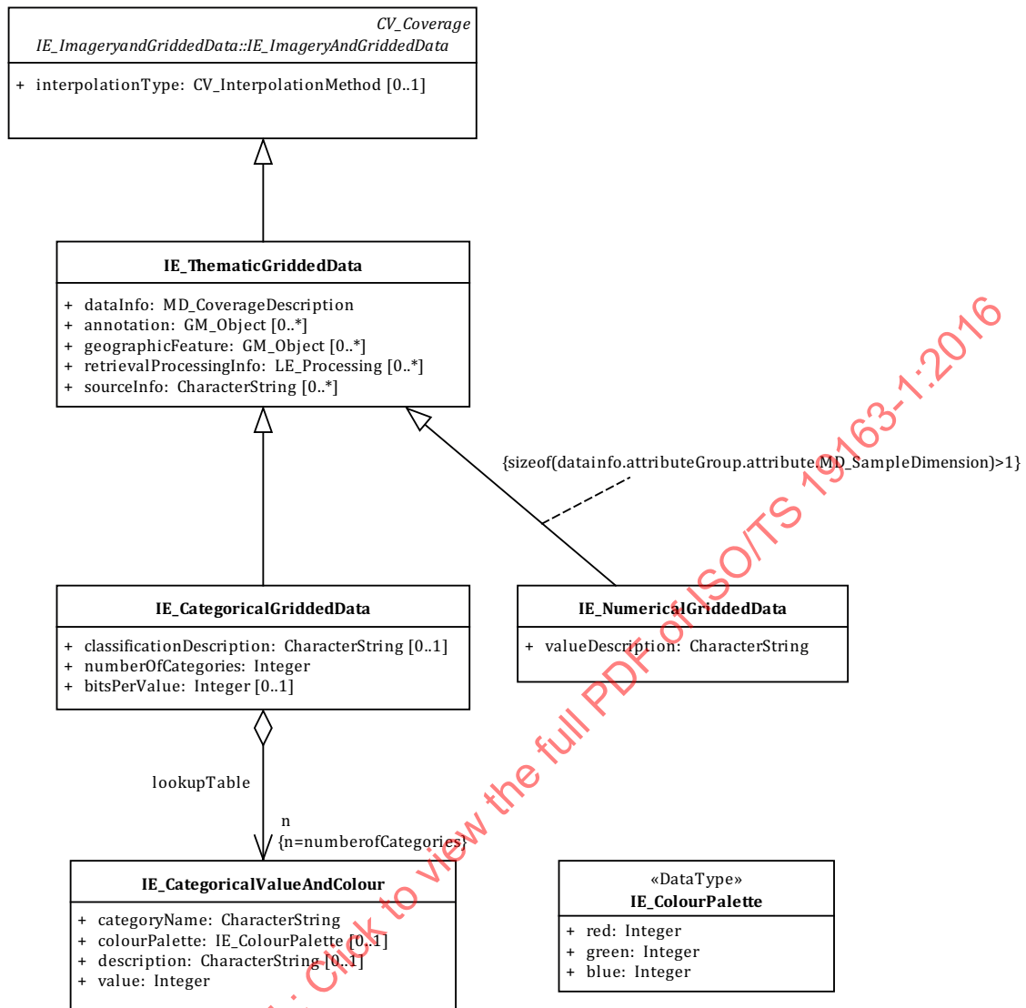
Figure 4 — IE_ThematicGriddedData
