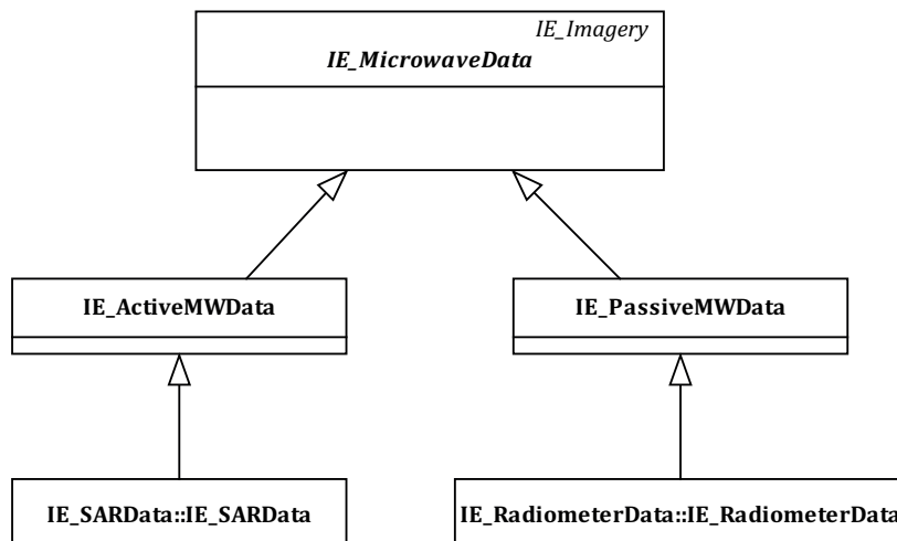
Figure 7 — IE_MicrowaveData
