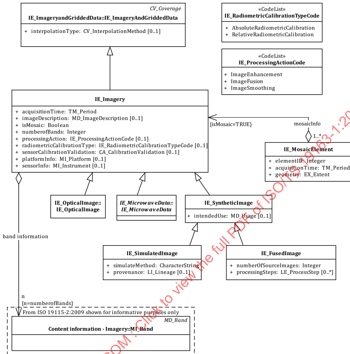
Figure 5 — IE_Imagery
