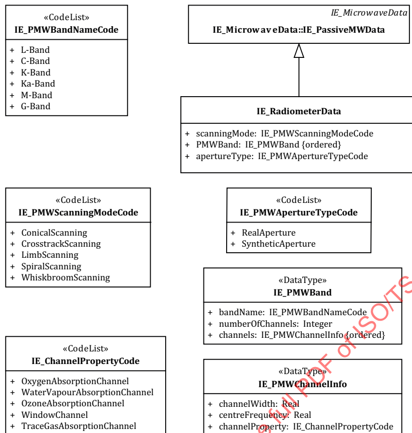
Figure 9 — IE_PassiveMWData
