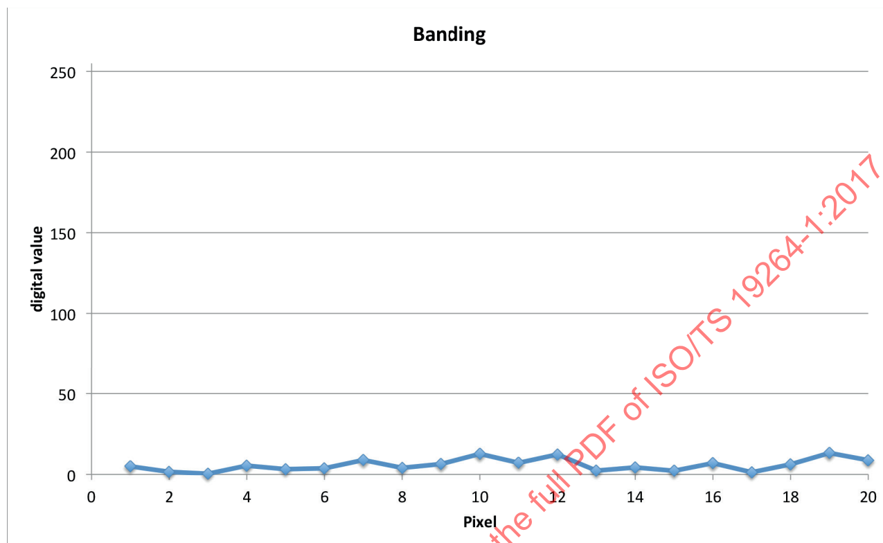
Figure 5 — Digital values over Pixels. Regular peaks in this structure indicate the presence of banding in images
