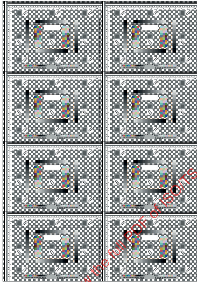
Figure C.4 — 8 targets combined into one A0 chart
