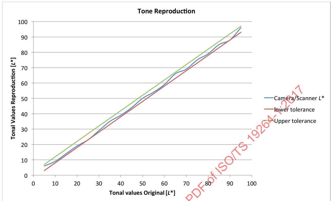
Figure 2 — Graphical representation for the tone reproduction
