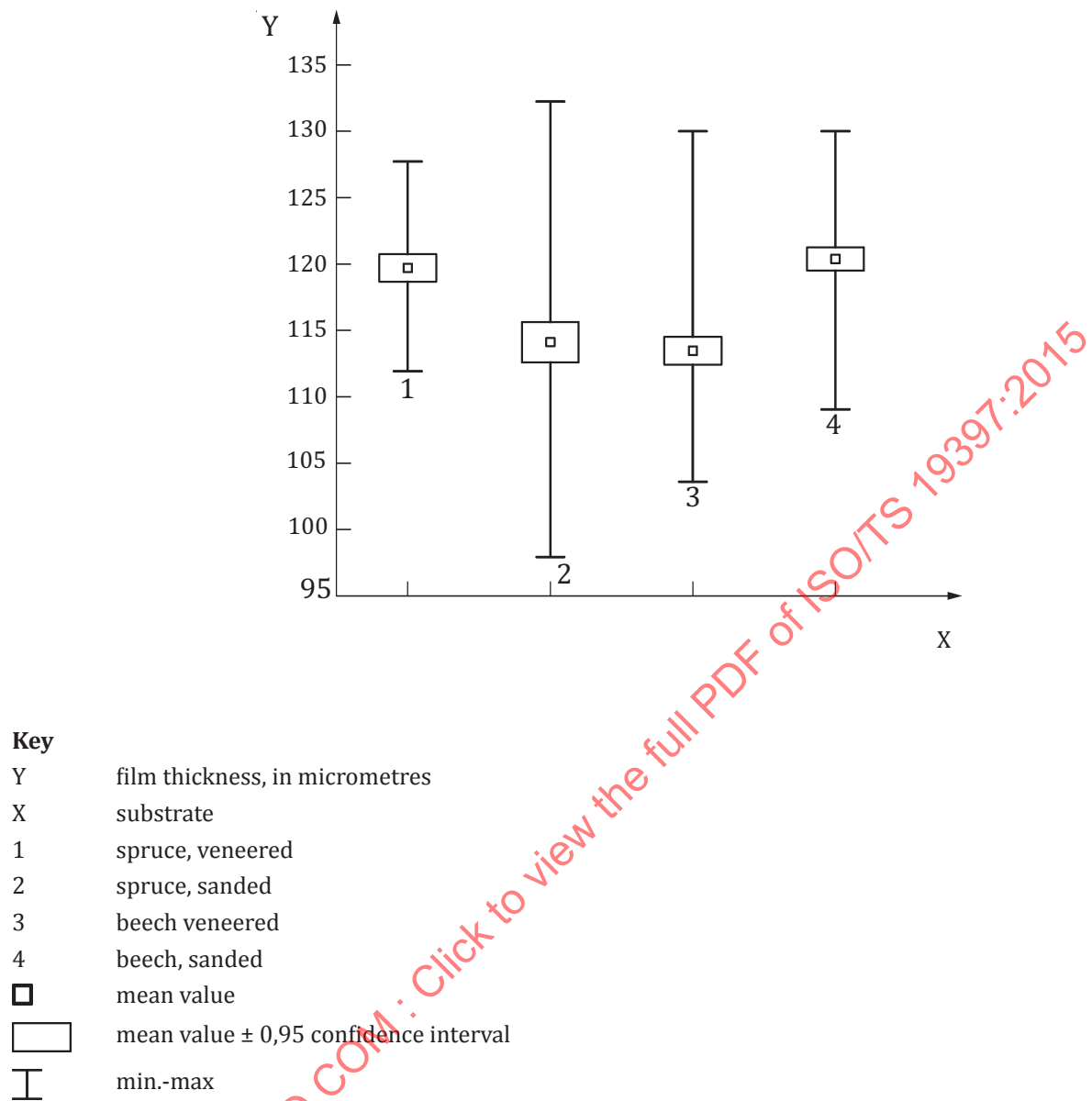
Figure B.1 — Diagram of the repeatability limit of the wood test specimens with a film thickness of 100 µm
