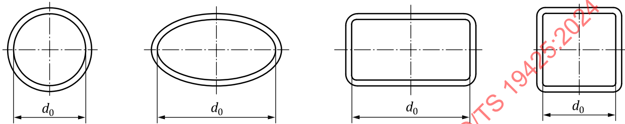
Figure 2 — Characteristic source dimension d_0 of typical air inlet (schematic)
