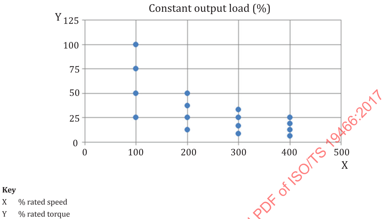
Figure 3 — Measurement points based on rated power
