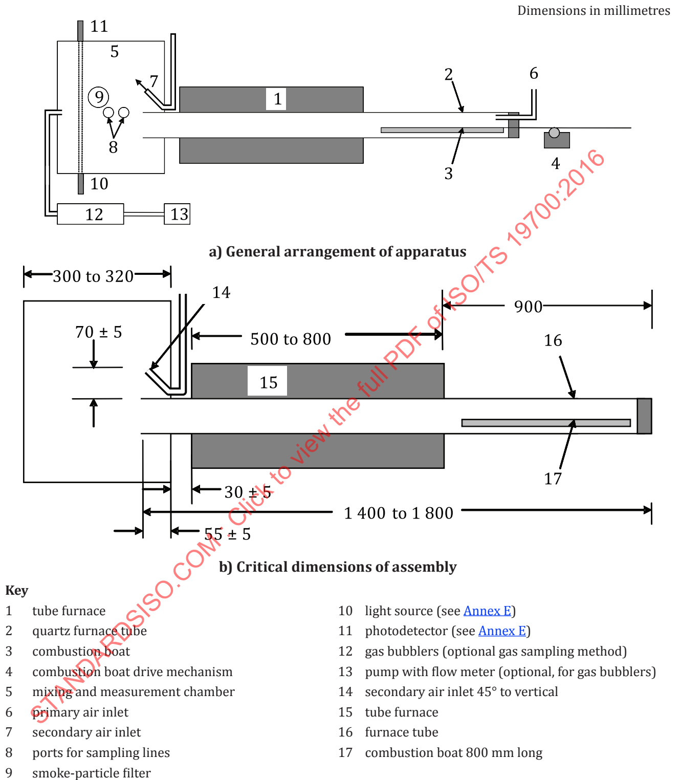
Figure 1 — Tube-furnace decomposition and sampling apparatus
