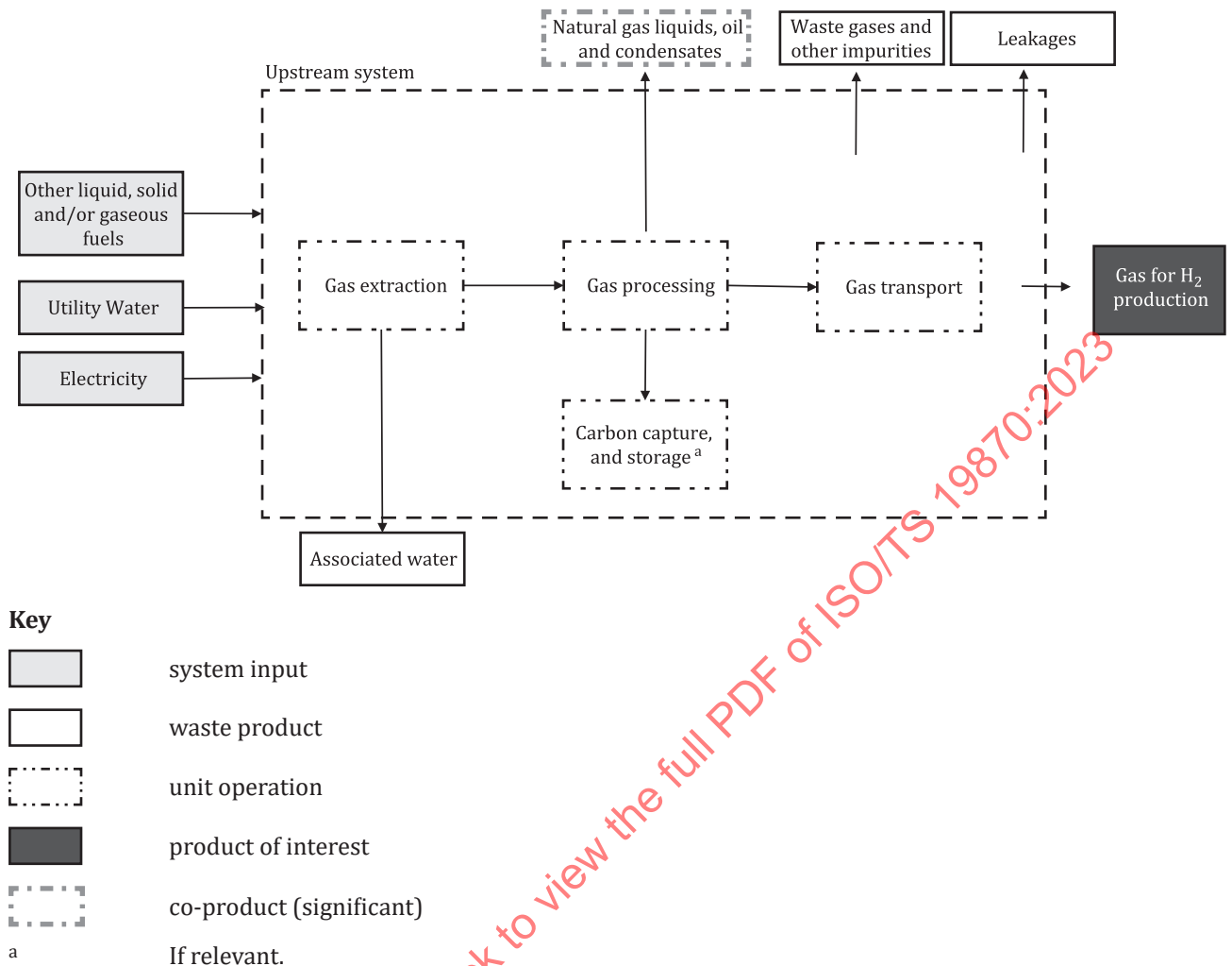
Figure 6 — Example of process diagram for the upstream system to deliver the natural gas for H 2 production
