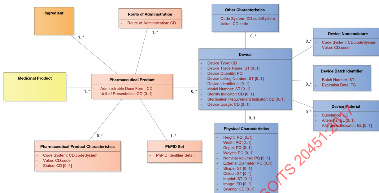
Figure B.1 — Pharmaceutical product and device section detailed description diagram
