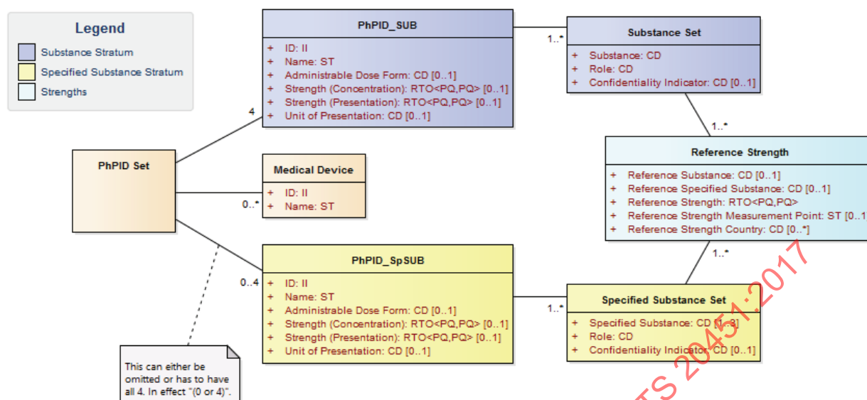
Figure 1 — Detailed model of the pharmaceutical product identification (PhPID)
