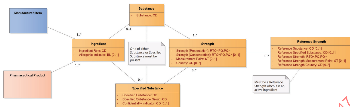
Figure A.1 — Ingredients, substance and strength section detailed description diagram
