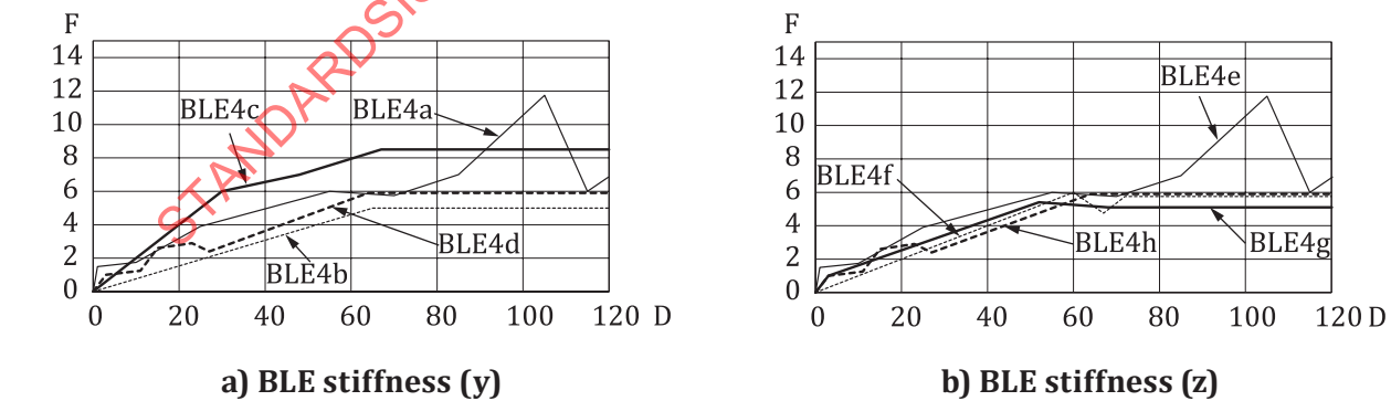
Figure A.28 — Force-deflection curves specified for the bumper and spoiler of the four J high-bumper SUV SCMs
