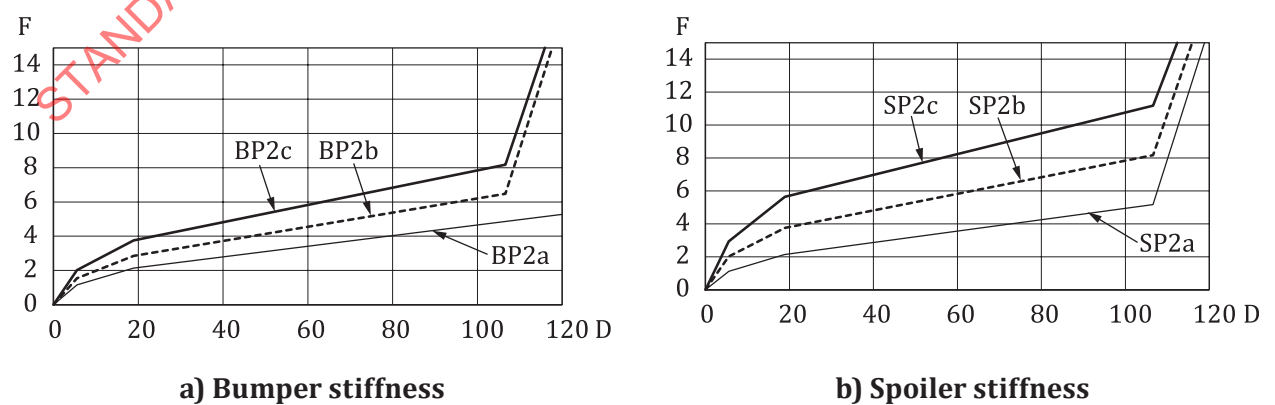
Figure A.25 — Force-deflection curves specified for the bumper and spoiler of the six J sedan SCMs
