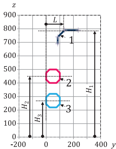
Figure B.5 — SCM with representative car shape for sedan with simple structures
