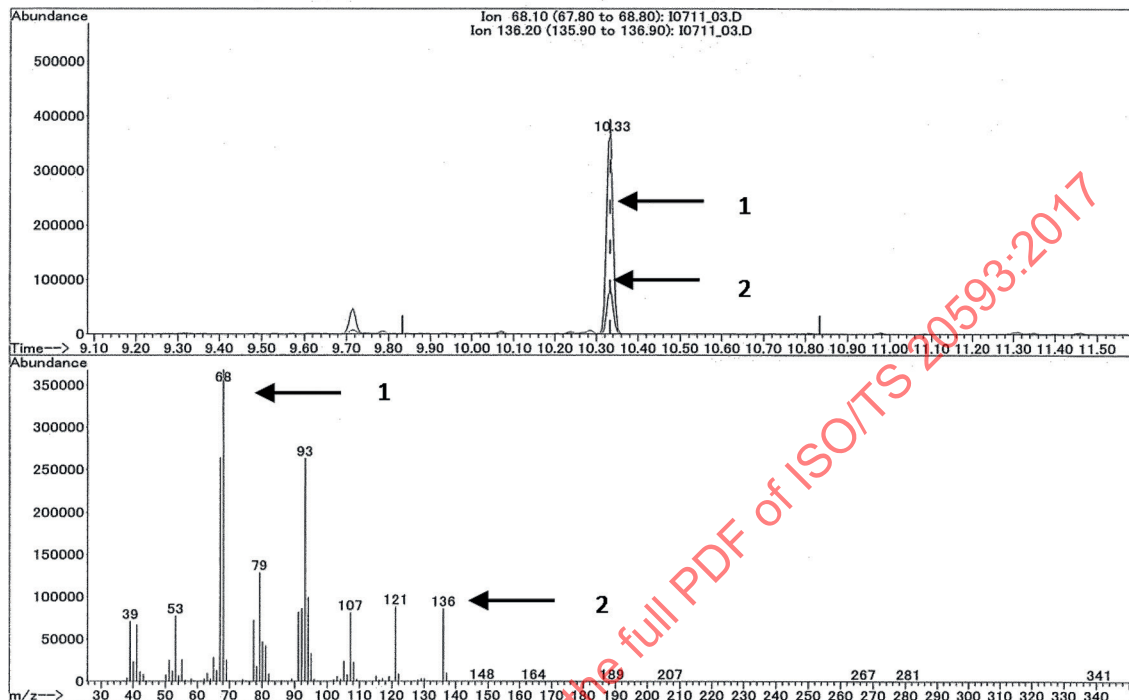
a) IpD peak from IR calibration standard
