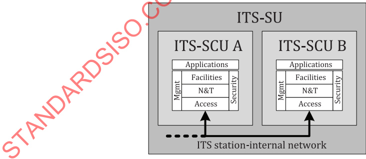
Figure 3 — Interconnection of ITS-SCUs in an ITS-SU
