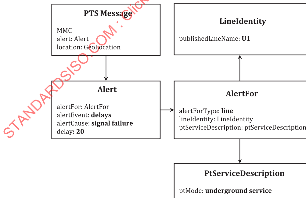
Figure C.2 — Alert for underground delays in both directions
