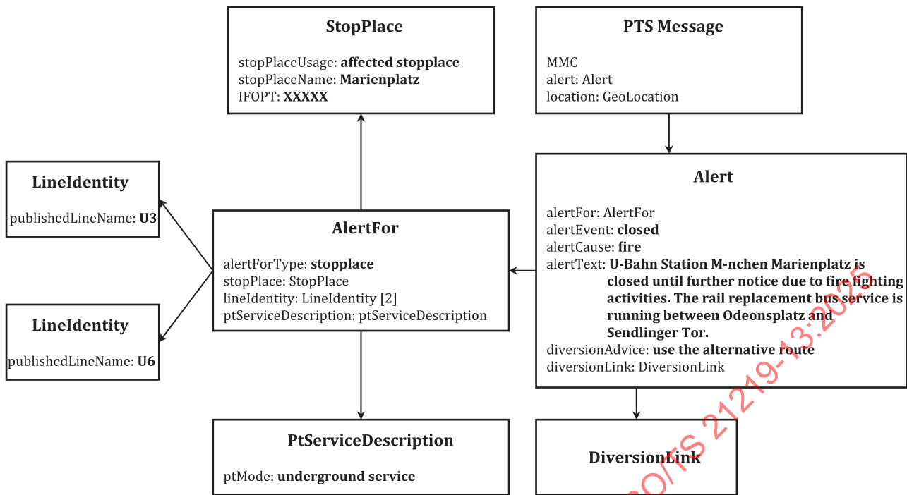
Figure C.1 — Alert for an underground station closure
