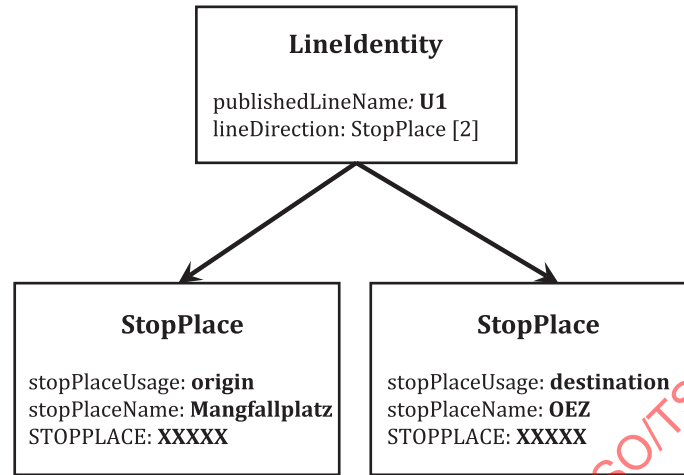
Figure C.3 — Alert for underground delays in one direction: LineIdentity component
