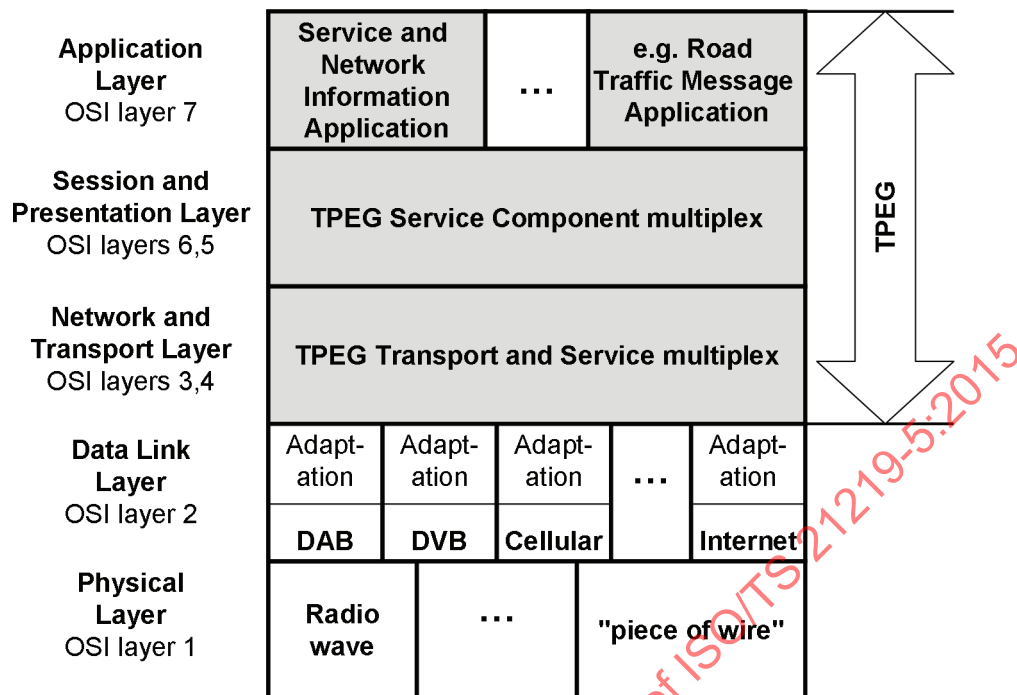
Figure 2 — TPEG in relation to the ISO/OSI Layer Model
