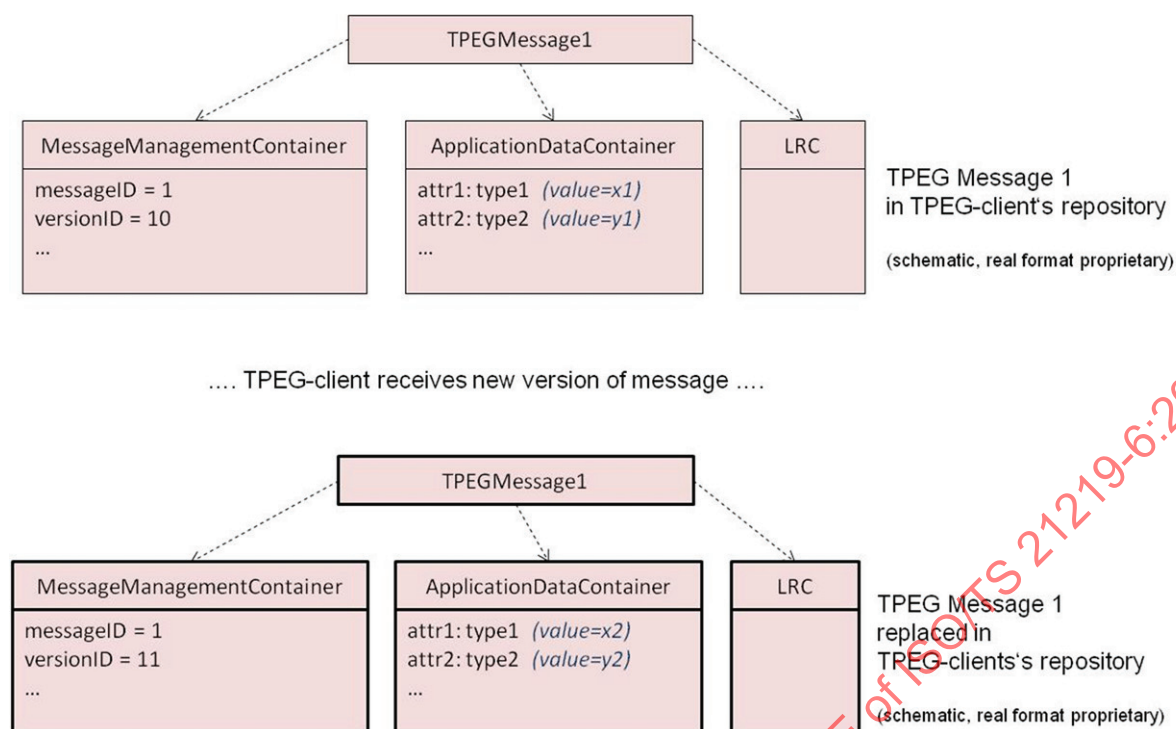
Figure 3 — Replacement of an overall message by Monolithic Message Management
