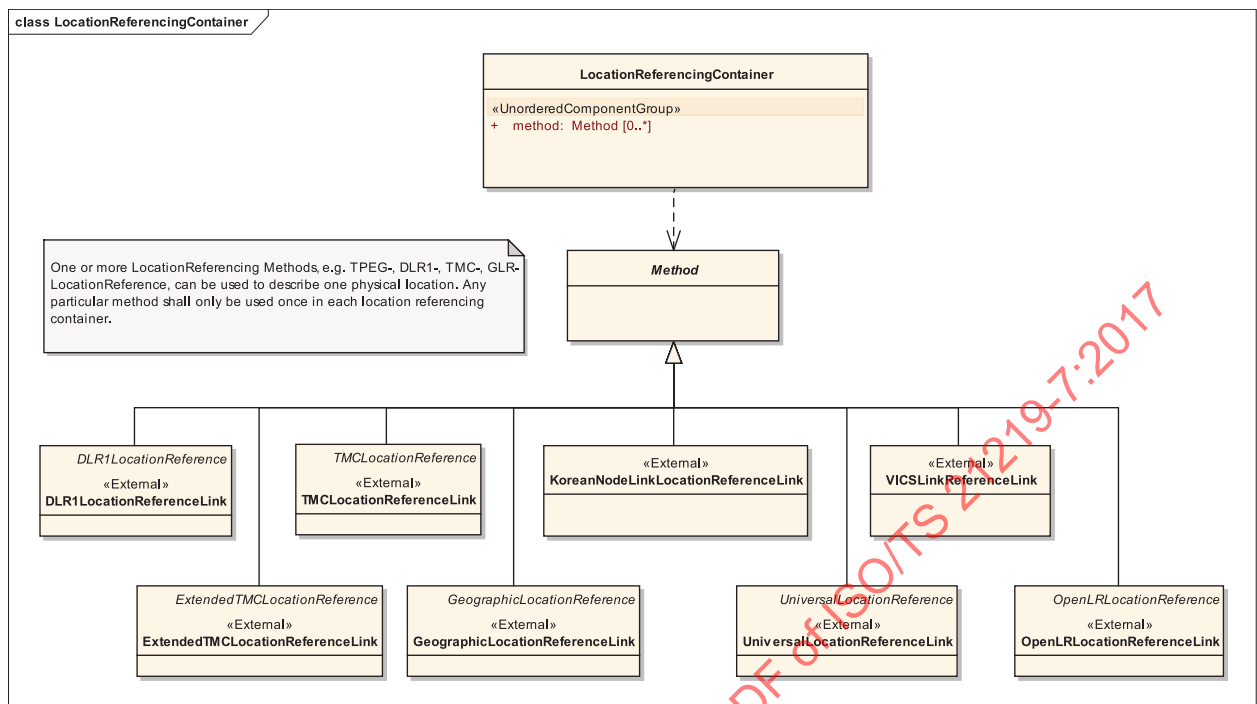
Figure 2 — LRC message structure
