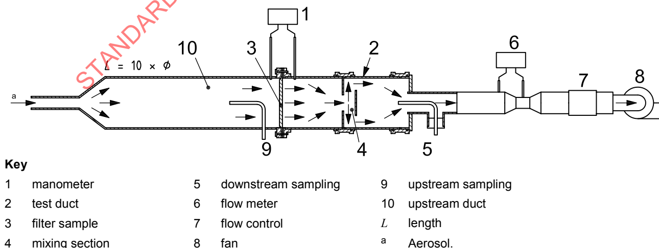
Figure A.1 — Filter material test equipment
