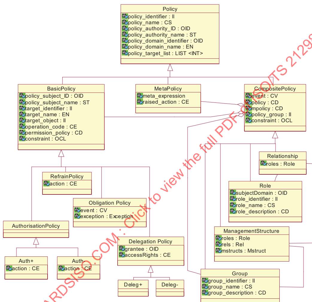
Figure 5 — Policy model
