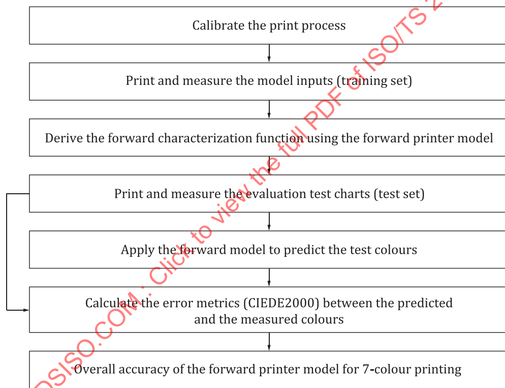
Figure A.1 — Processing steps
